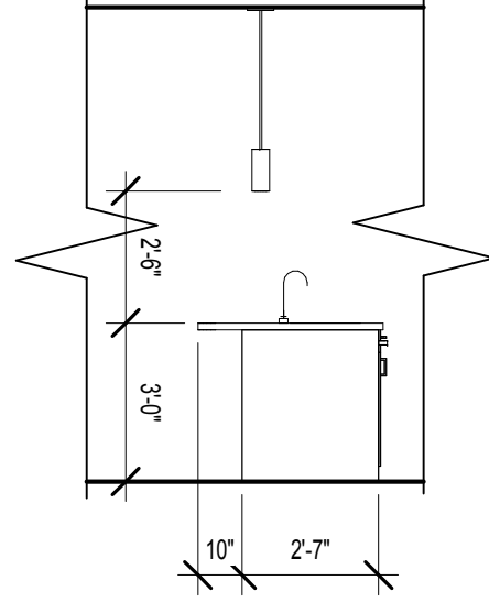
8 UNIT A1 - KITCHEN ISLAND ELEVATION SCALE: 1/4" = 1'-0"
