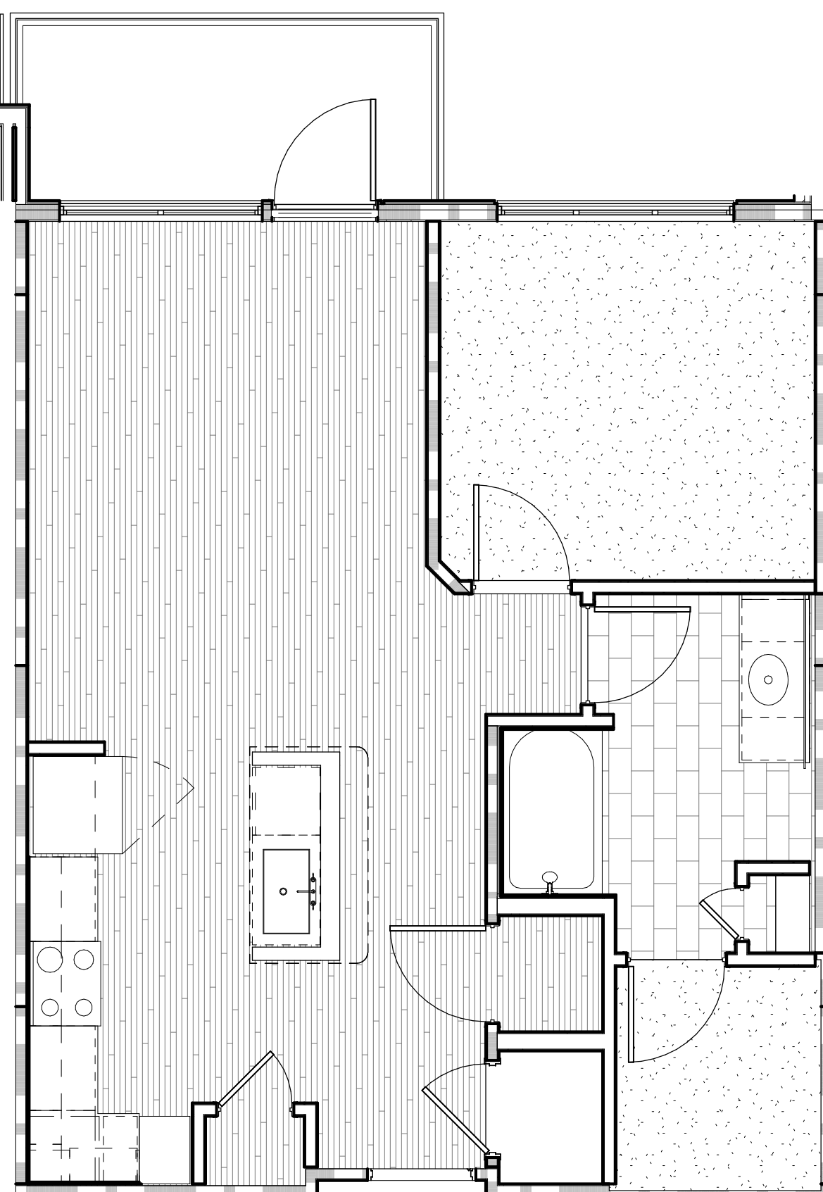
3 UNIT A1 FLOORING PLAN SCALE: 1/4" = 1'-0"
