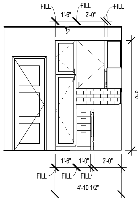
6 UNIT A1 - KITCHEN PANTRY ELEVATION SCALE: 1/4" = 1'-0"
