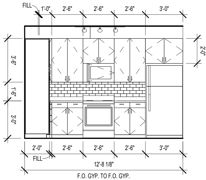
5 UNIT A1 - KITCHEN RANGE ELEVATION SCALE: 1/4" = 1'-0"
