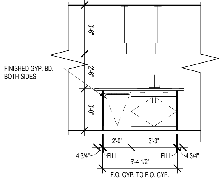
7 UNIT A1 - KITCHEN ISLAND SINK ELEVATION SCALE: 1/4" = 1'-0"
