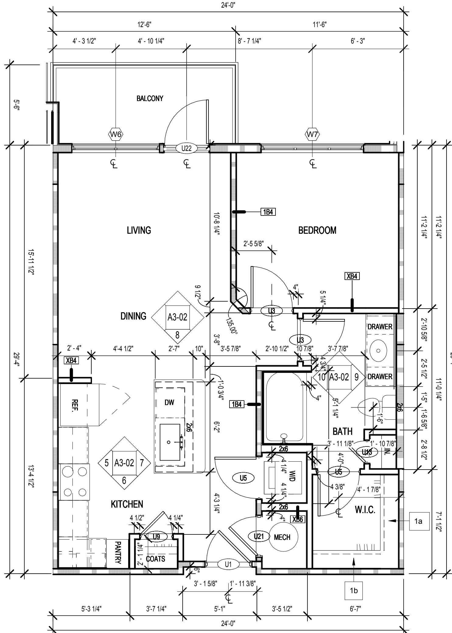
1 UNIT A1 FLOOR PLAN SCALE: 1/4" = 1'-0"
