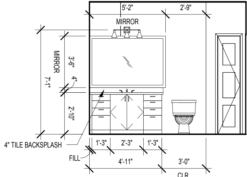
9 UNIT A1 - BATHROOM VANITY ELEVATION SCALE: 1/4" = 1'-0"
