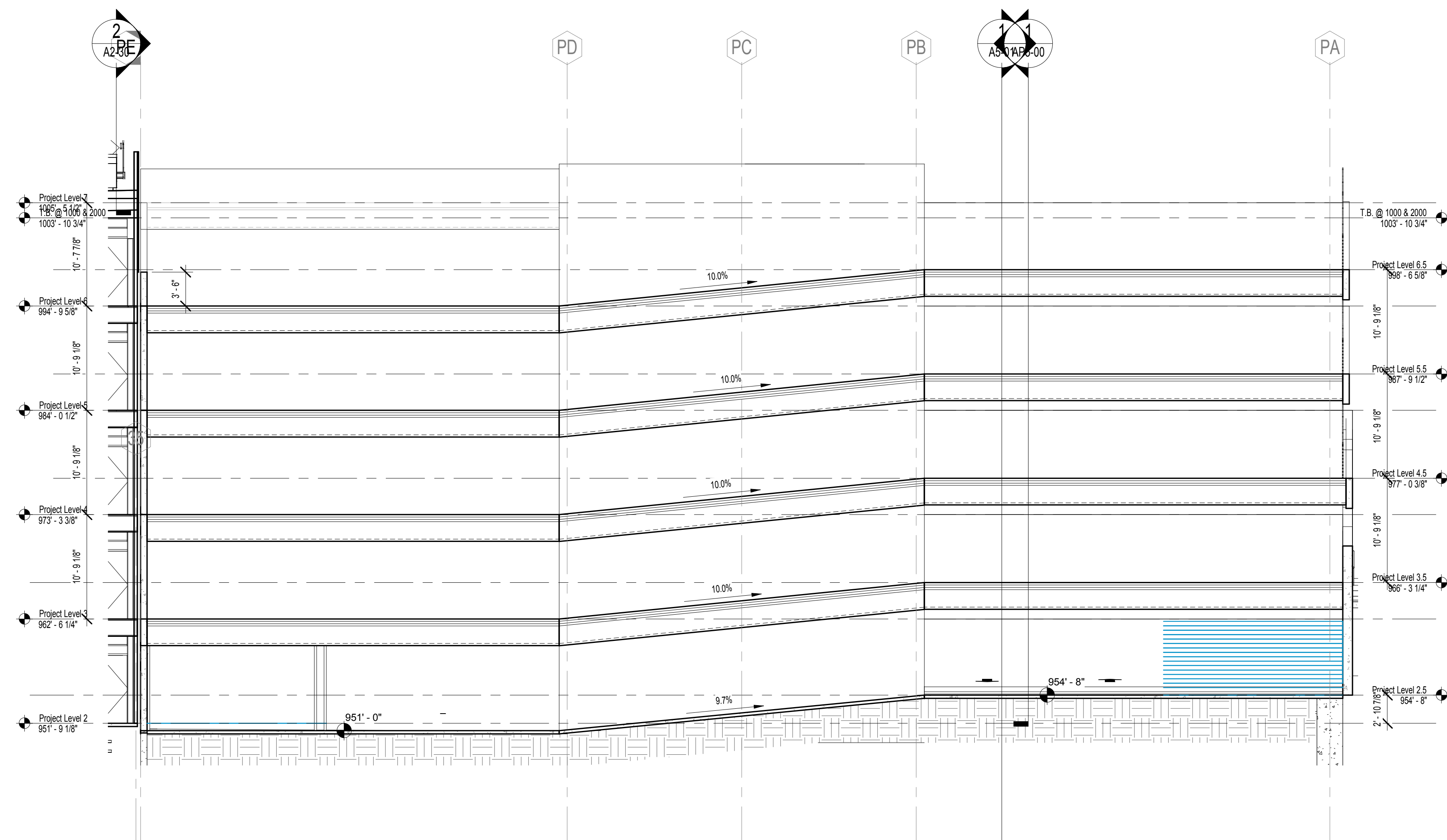
2 PARKING DECK SECTION 2 SCALE: 1/8" = 1'-0"
