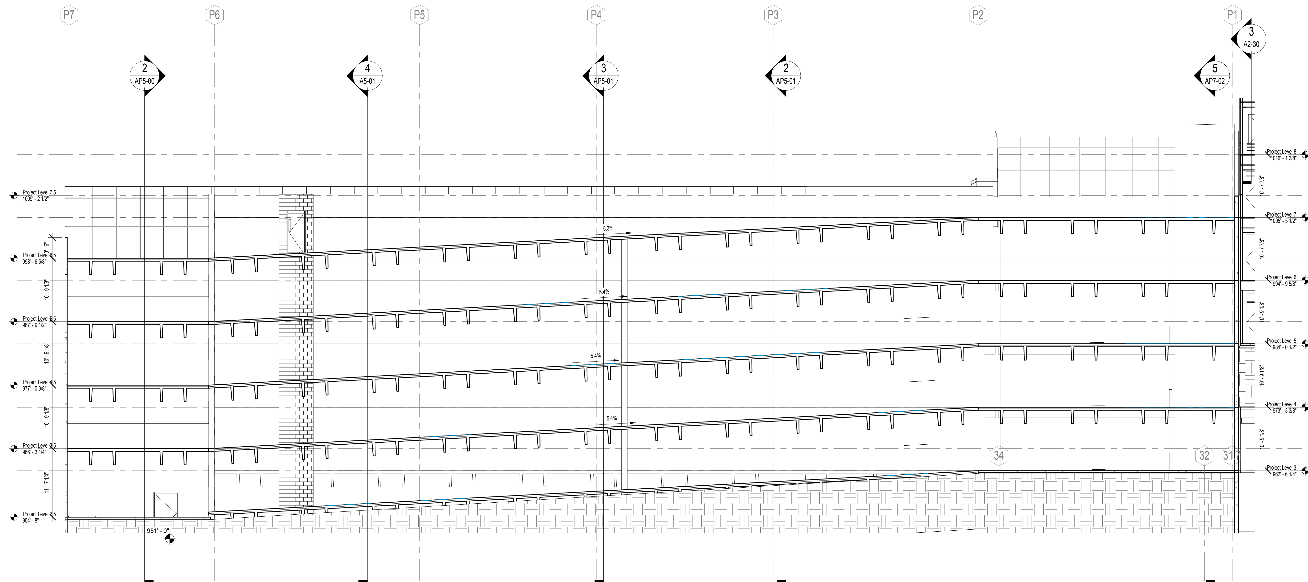
1 PARKING DECK SECTION 1 SCALE: 1/8" = 1'-0"
