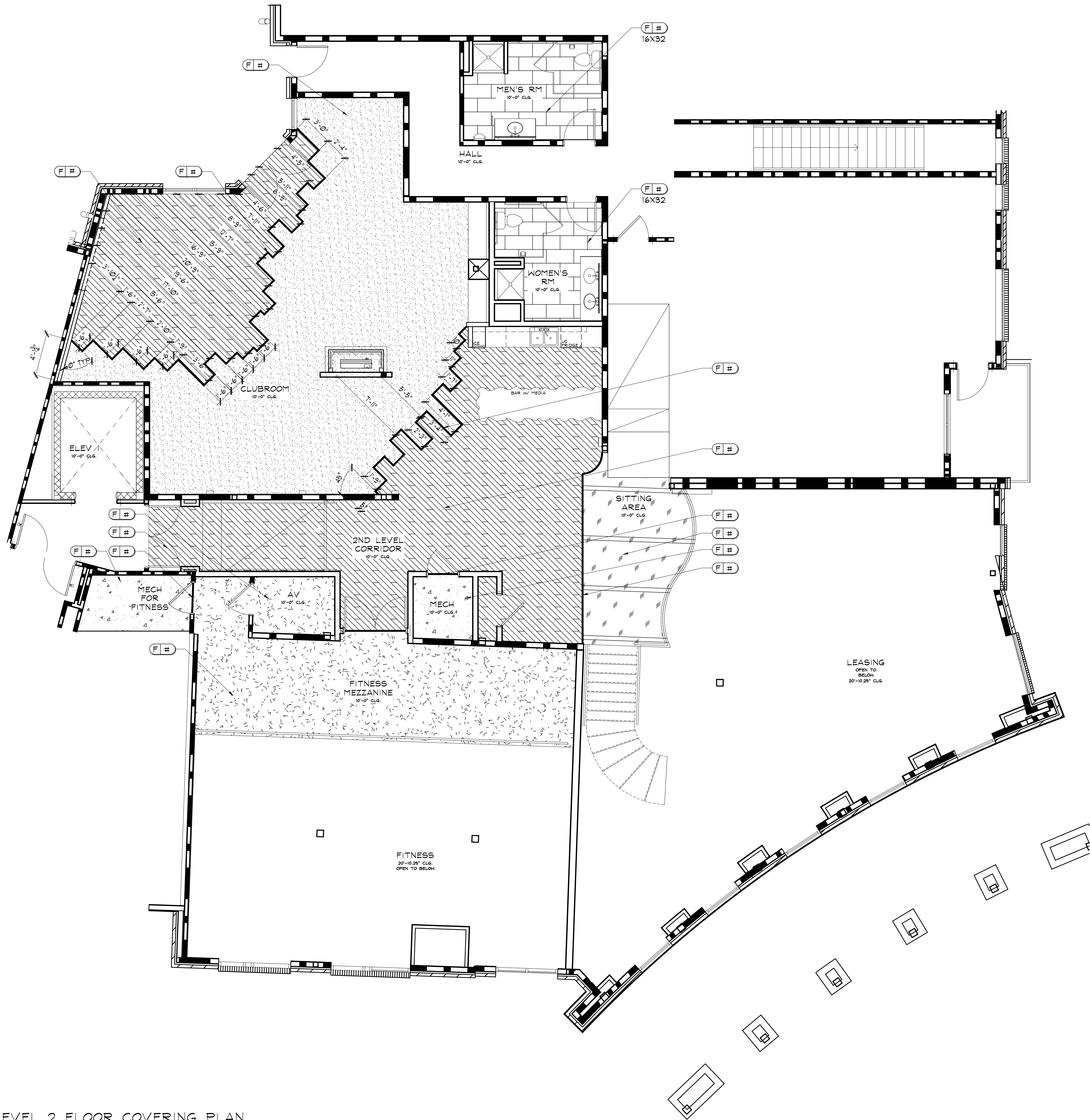
1 LEVEL 2 FLOOR COVERING PLAN ID.401 SCALE : 1/4" = 1'-0"
