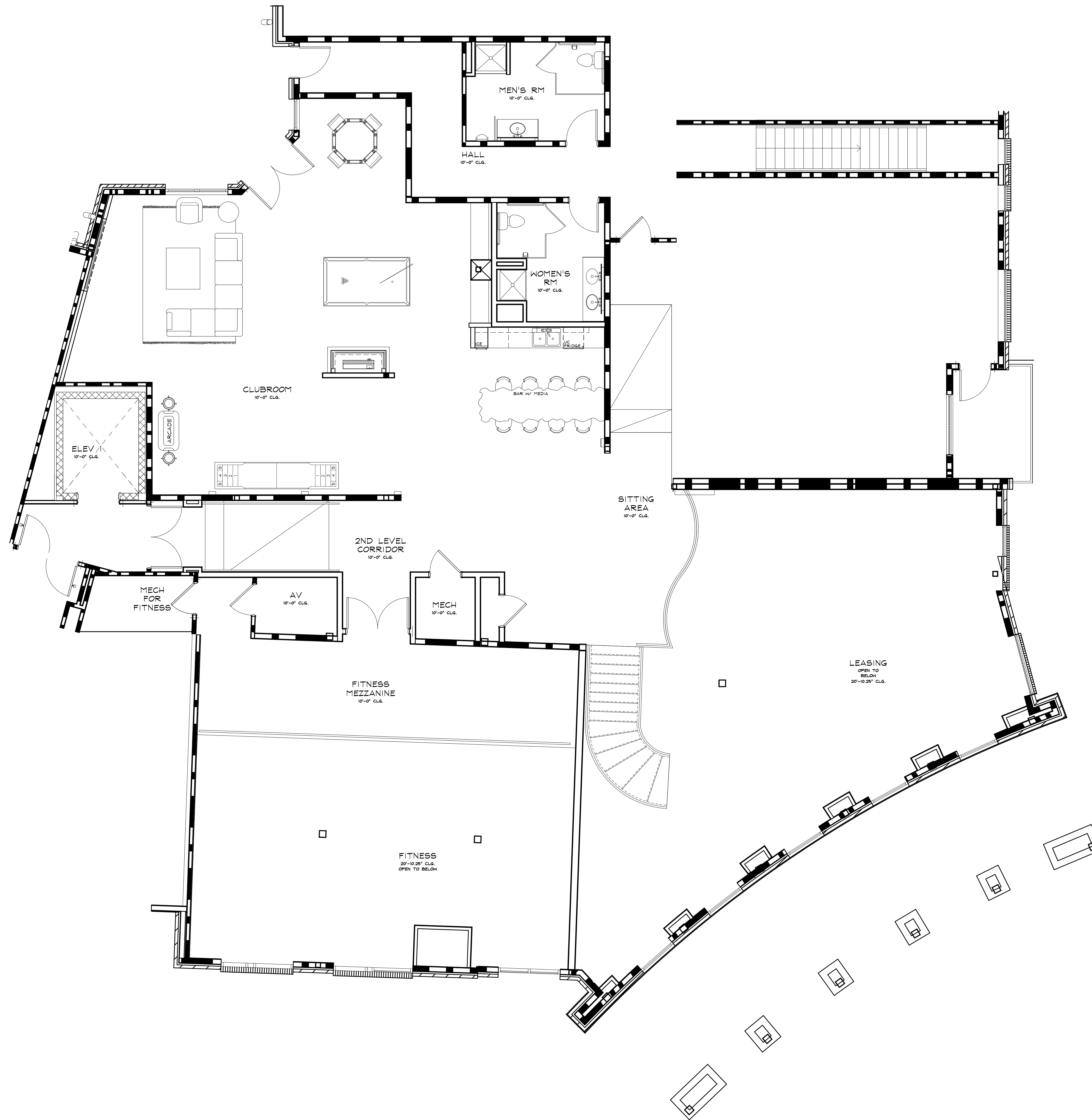
1 LEVEL 1 FURNITURE AND FIXTURES PLAN ID.501 SCALE : 1/4" = 1'-0"
