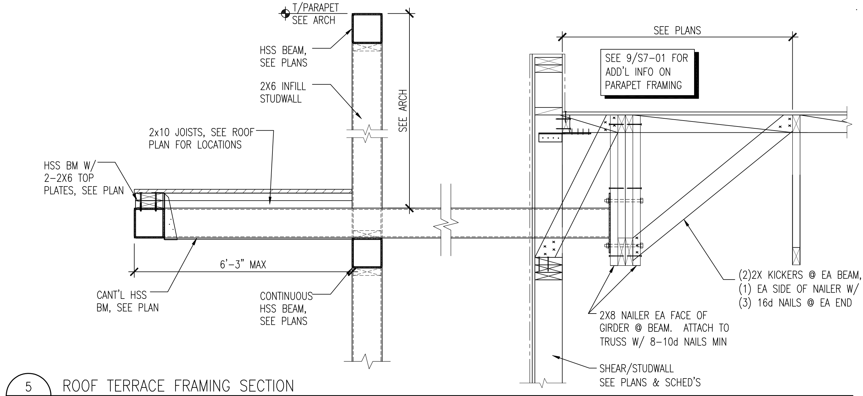
5 ROOF TERRACE FRAMING SECTION S7-02 SCALE: 1" = 1'-0"
