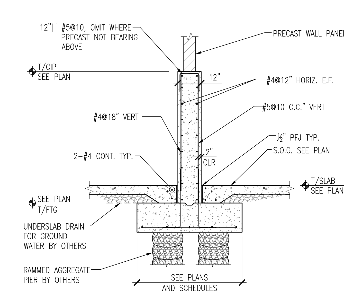
3 SECTION AT PRECAST BEARING ON CIP WALL SCALE: 3/8" = 1'-0"
