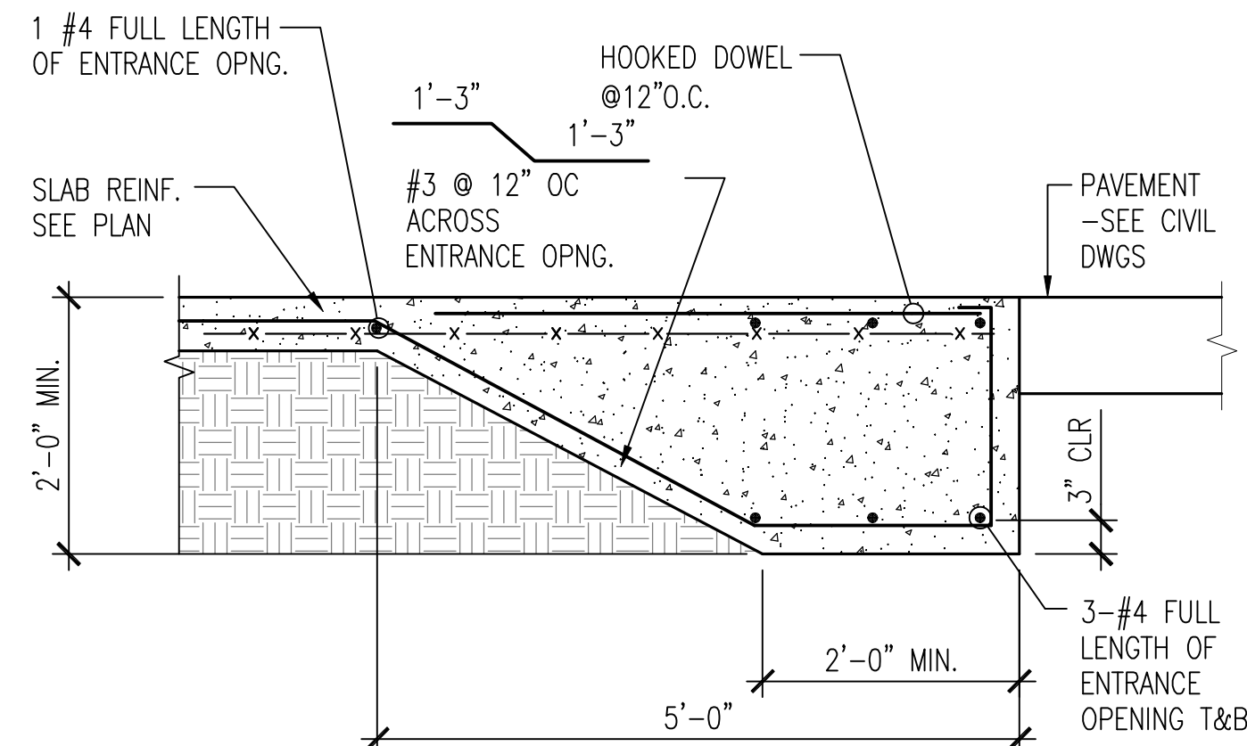
9 TYP. EXTERIOR SLAB DETAIL @ ENTRANCE SCALE: 3/4" = 1'-0"
