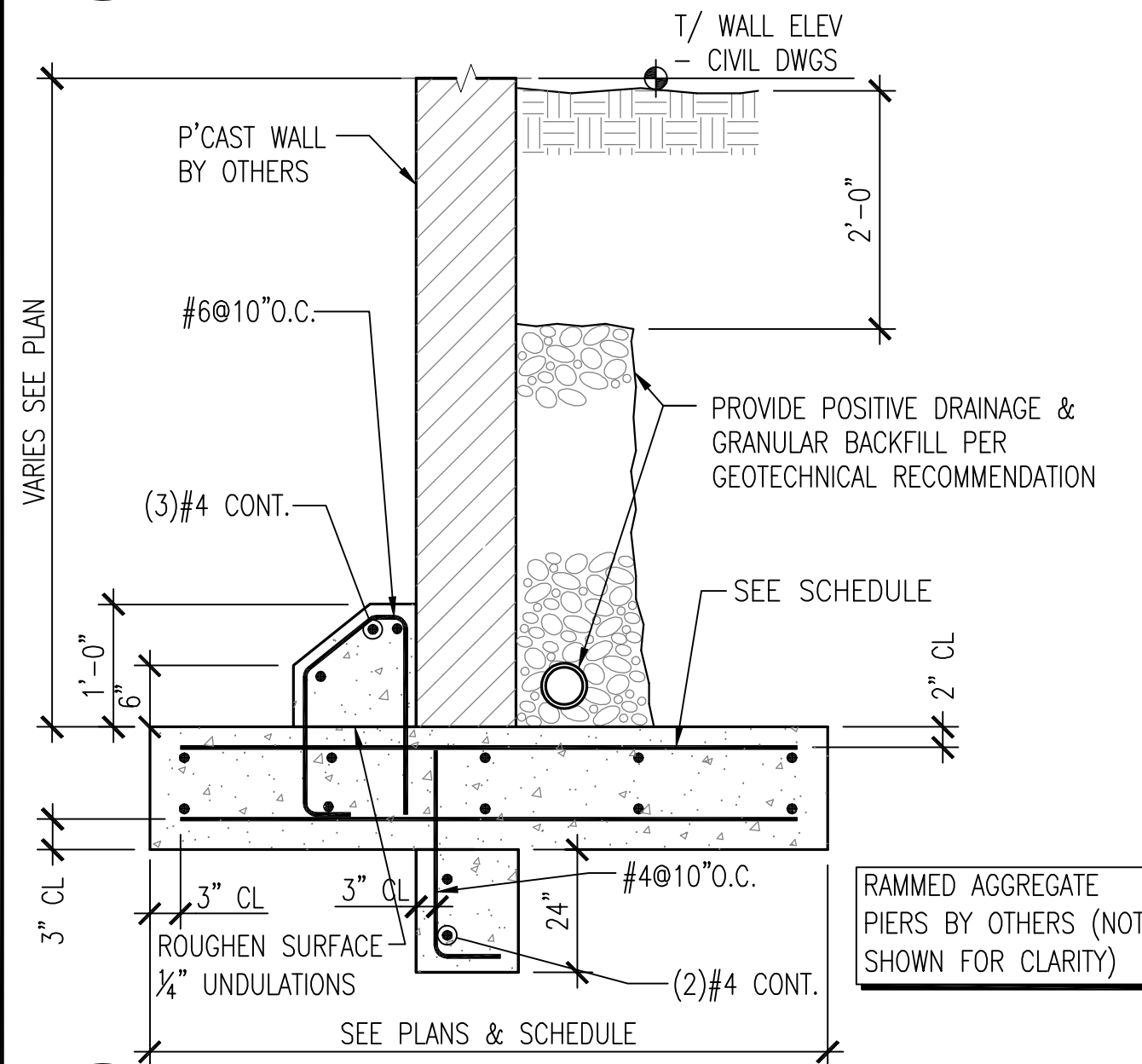
18 SITE RETAINING WALL SCALE: 3/4" = 1'-0"
