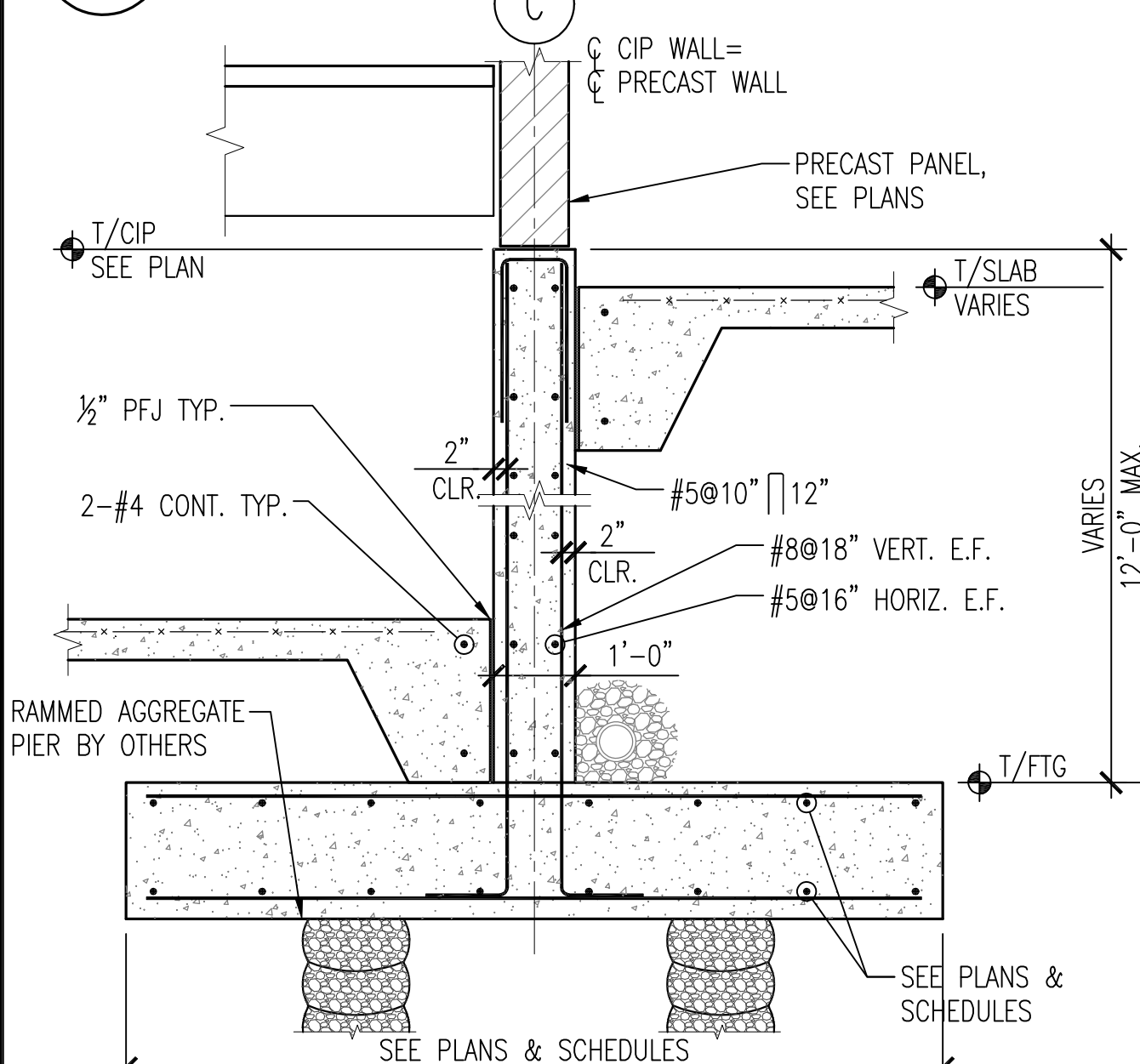
19 SECTION RETAINING WALL W/ PRECAST SCALE: 1/2" = 1'-0"
