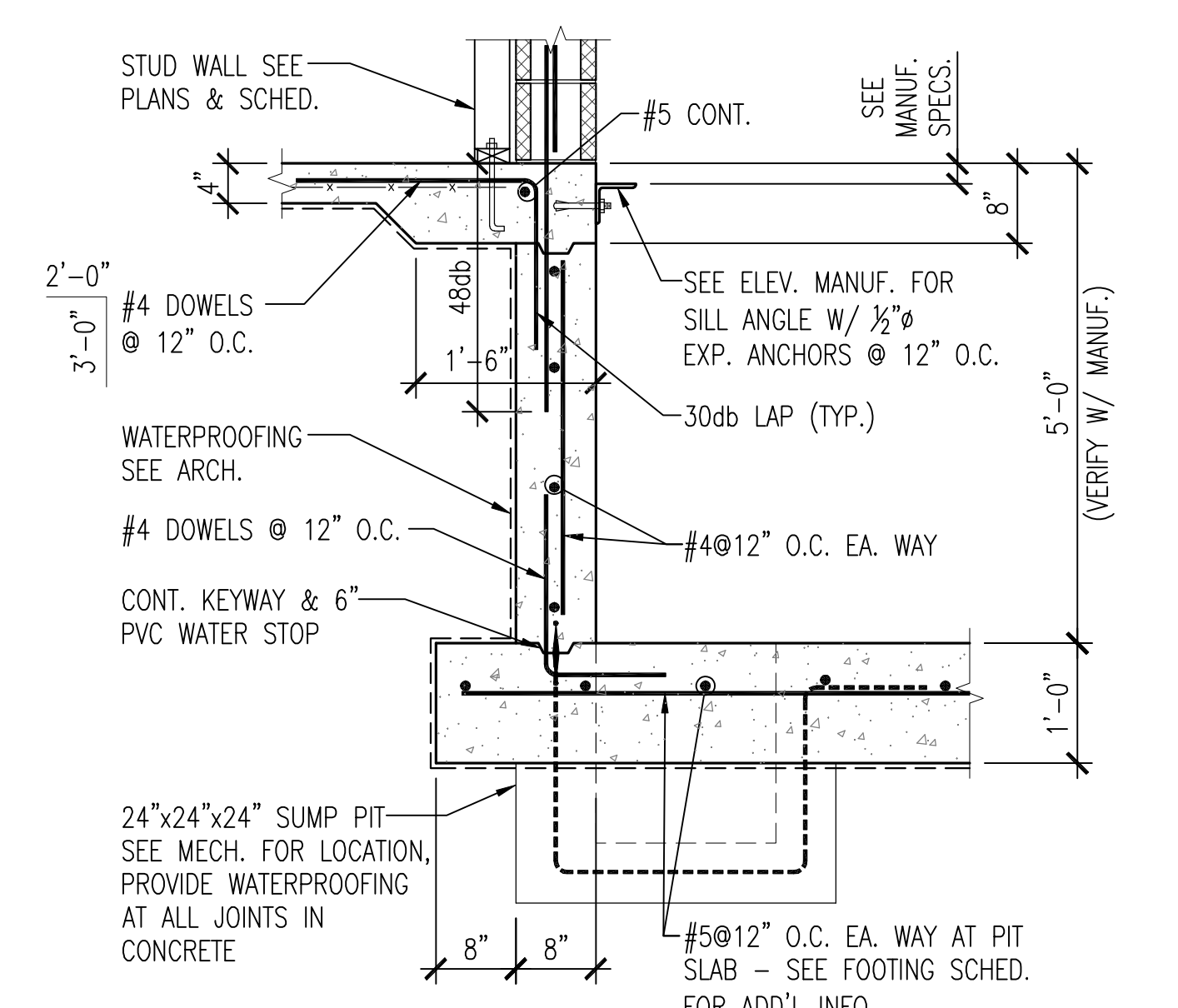
4 TYPICAL DETAIL - SECTION AT ELEVATOR PIT SCALE: 3/4" = 1'-0"
