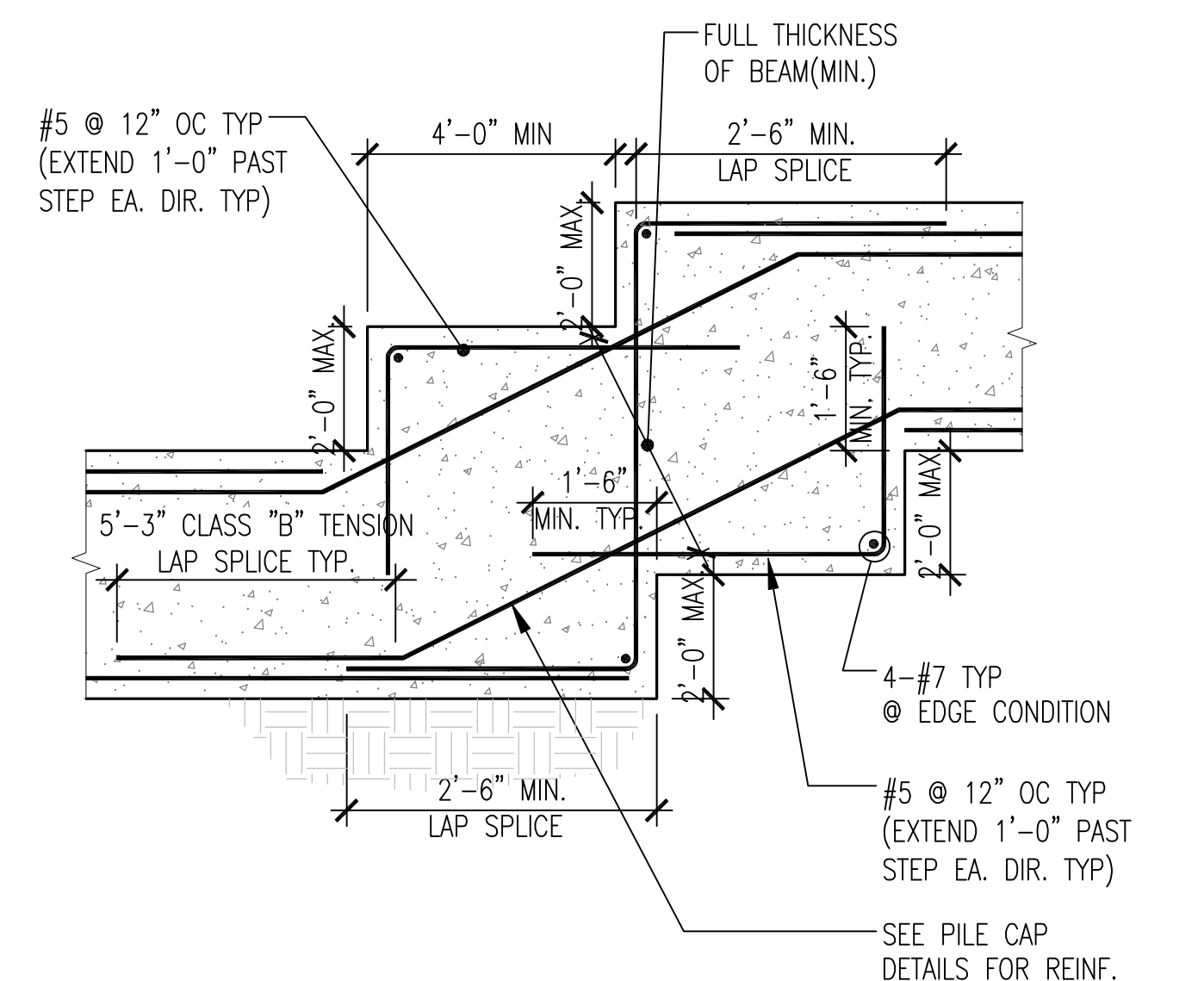
10 TYP. STEPPED GRADE BM DETAIL SCALE: 3/4" = 1'-0"
