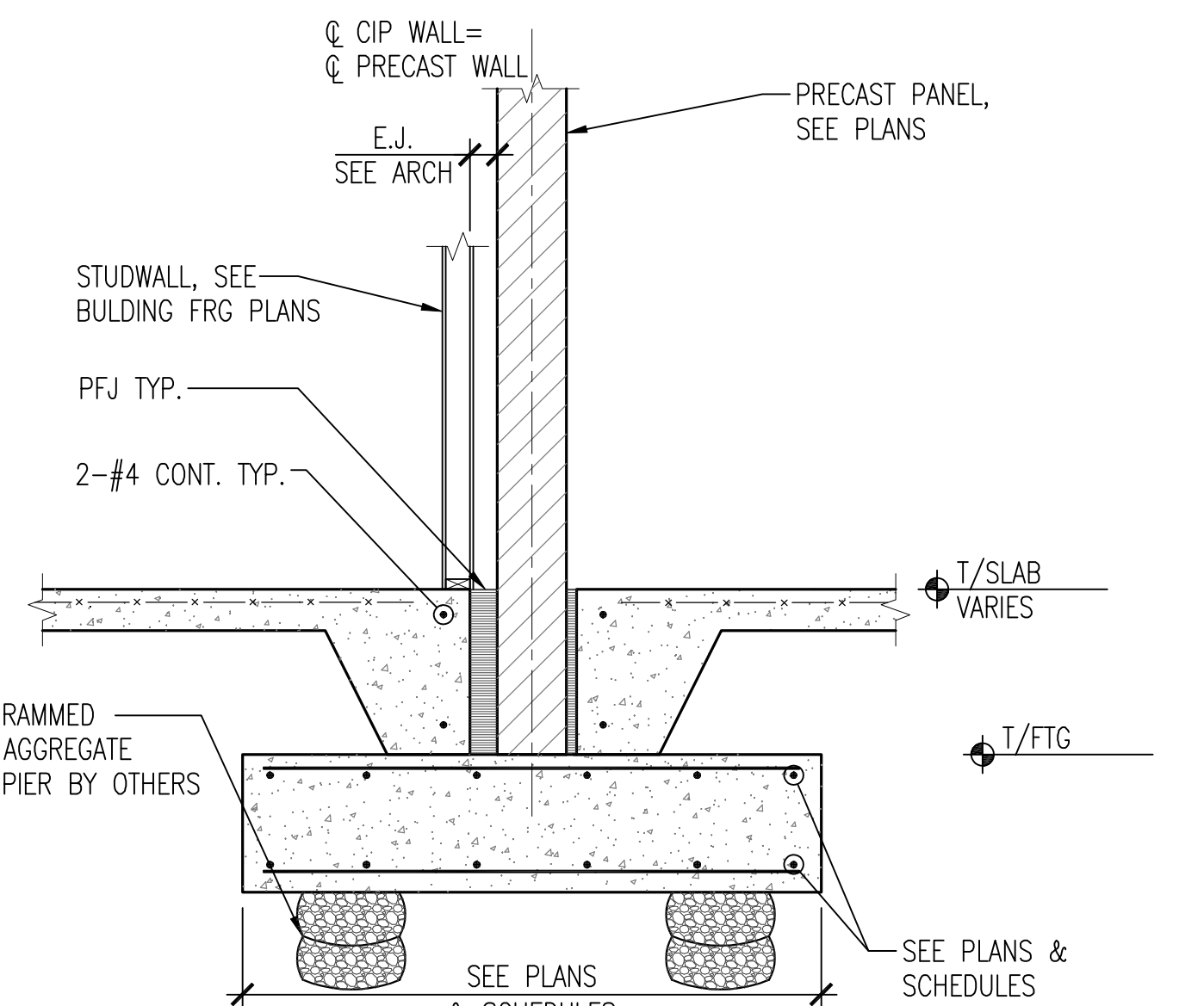
11 SECTION AT PRECAST BEARING SCALE: 1/2" = 1'-0"
