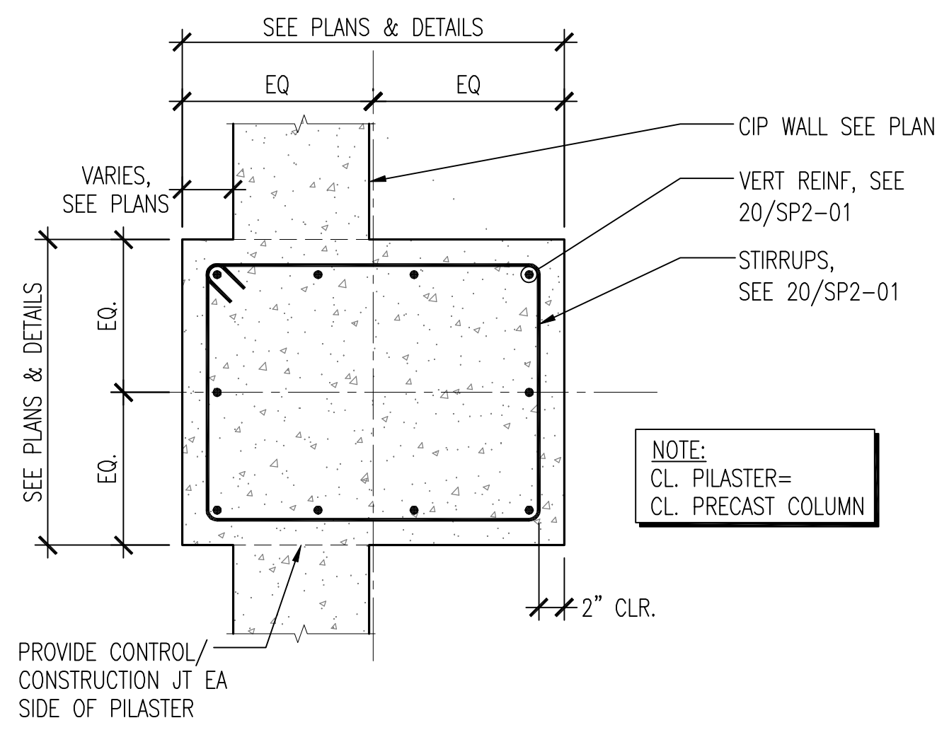
6 PLAN DETAIL AT PILASTER SCALE: 3/4" = 1'-0"
