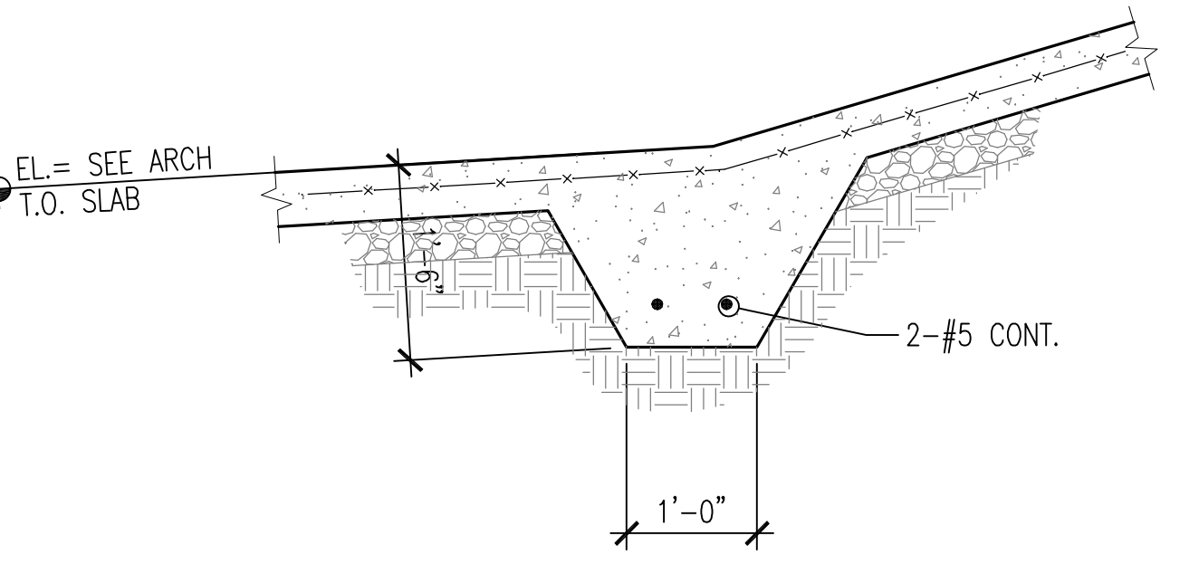
8 TYPICAL DETAIL - RAMP ON GRADE SCALE: 3/4" = 1'-0"
