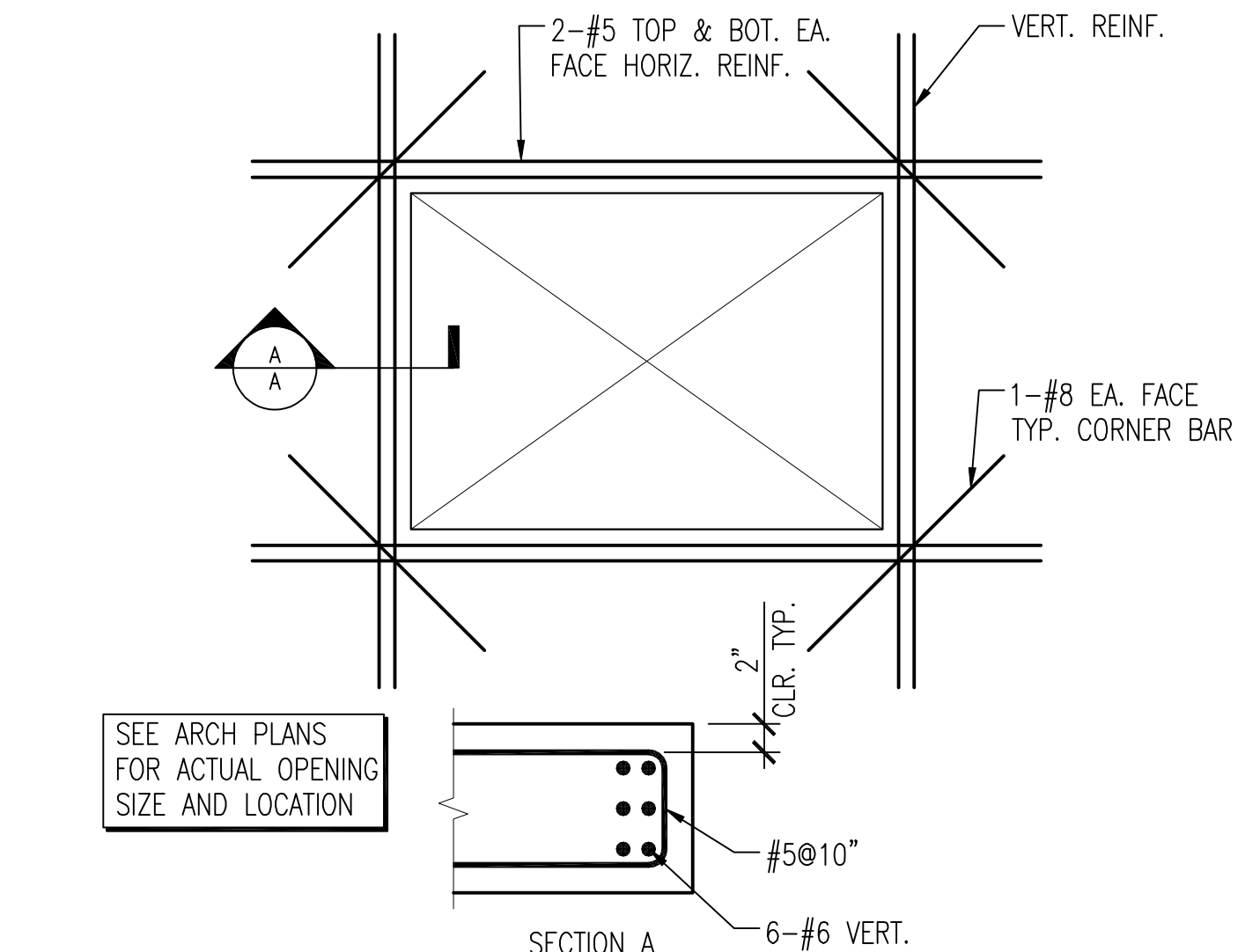
2 ADDITIONAL REINFORCEMENT AT OPENING IN CIP WALL SCALE: 1/2" = 1'-0"
