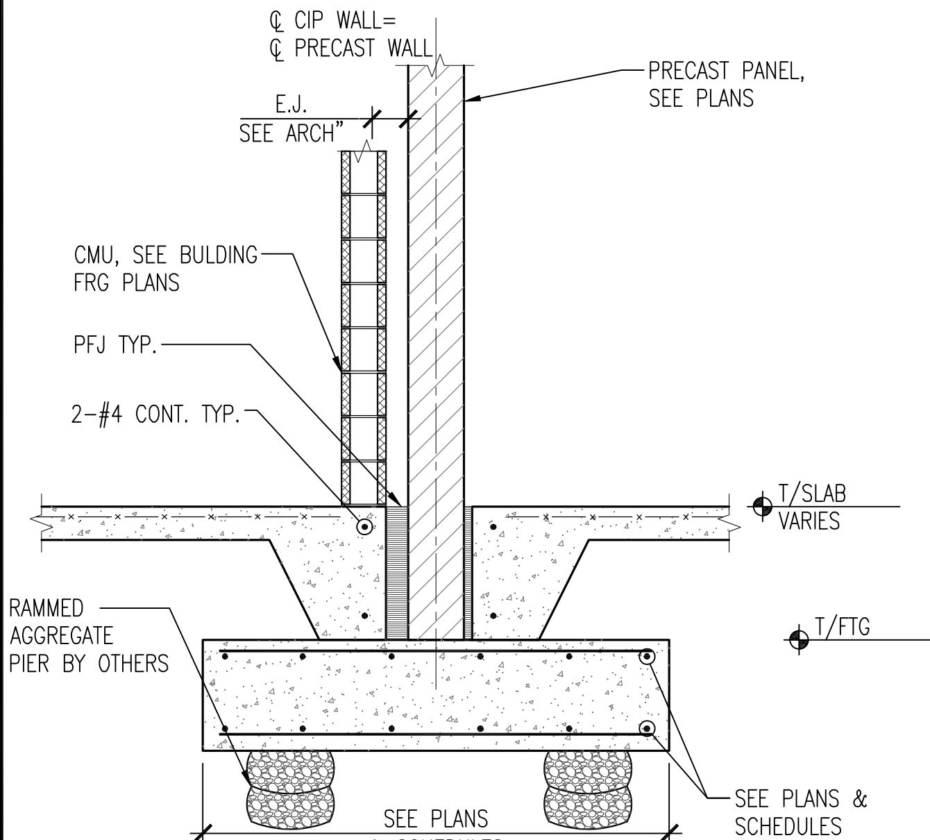
20 SECTION AT PRECAST BEARING SCALE: 1/2" = 1'-0"
