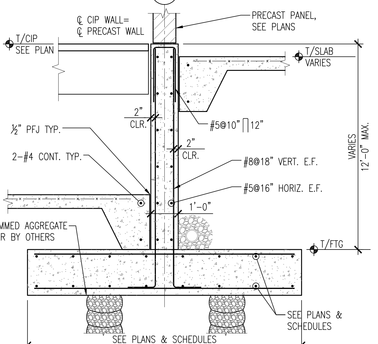
7 SECTION RETAINING WALL W/ PRECAST SCALE: 1/2" = 1'-0"
