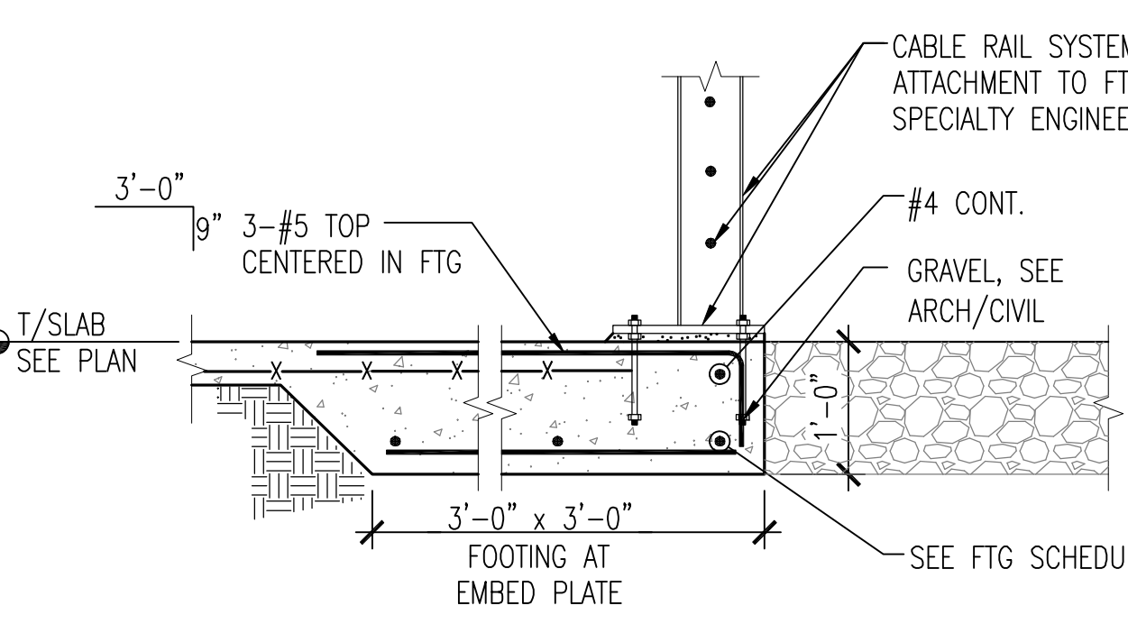
16 SECTION @ CABLE RAIL EMBED PLATE ON GRADE SCALE: 3/4" = 1'-0"
