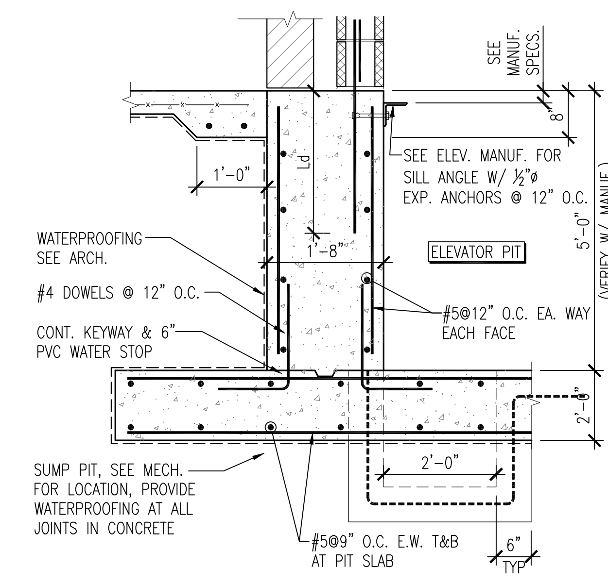
15 SECTION AT ELEVATOR PIT W/ PRECAST SCALE: 3/4" = 1'-0"
