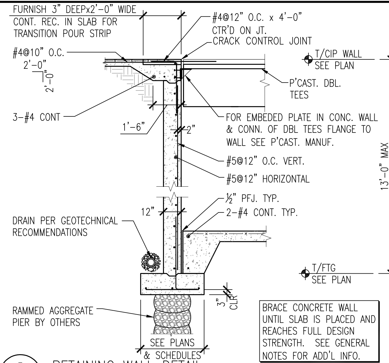
5 RETAINING WALL DETAIL SCALE: 3/8" = 1'-0"
