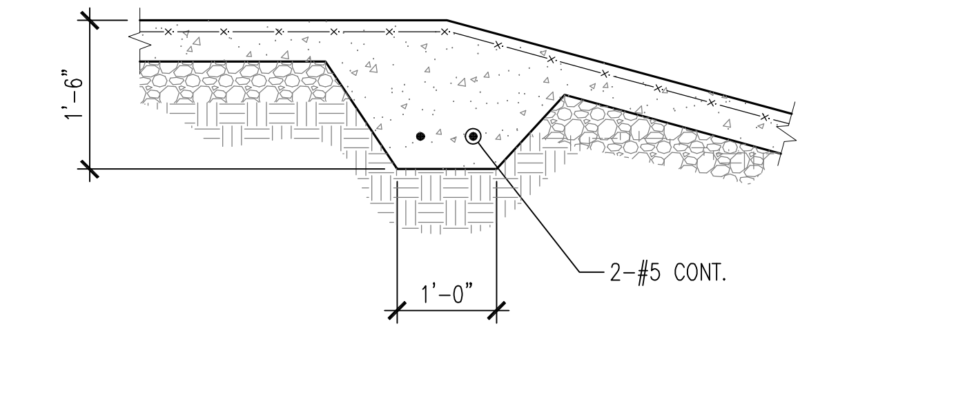
12 TYPICAL DETAIL - RAMP ON GRADE SCALE: 3/4" = 1'-0"
