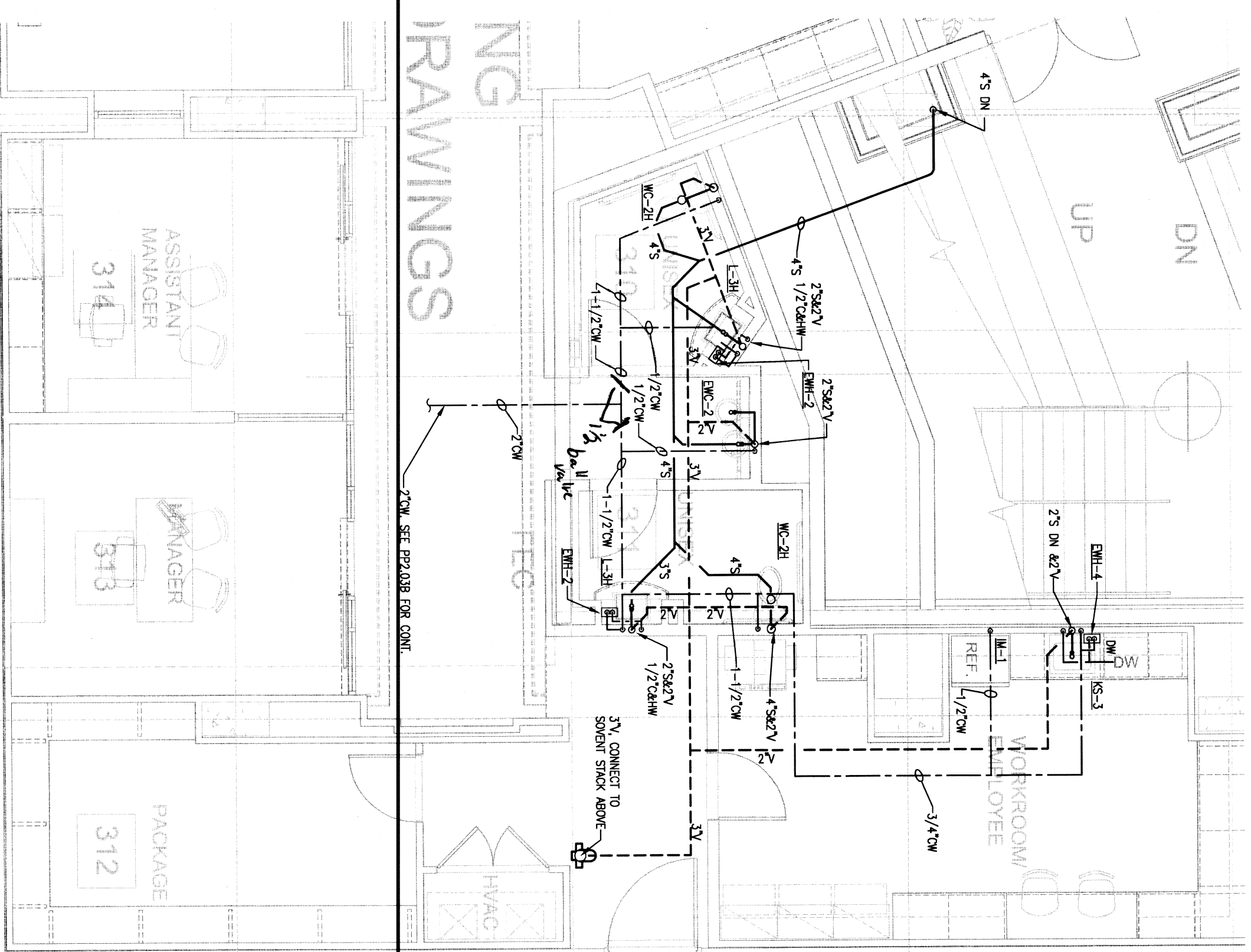
1 LEVEL 3, LEASING, PLUMBING PLAN P.L.O.T. 1/4\"/>
